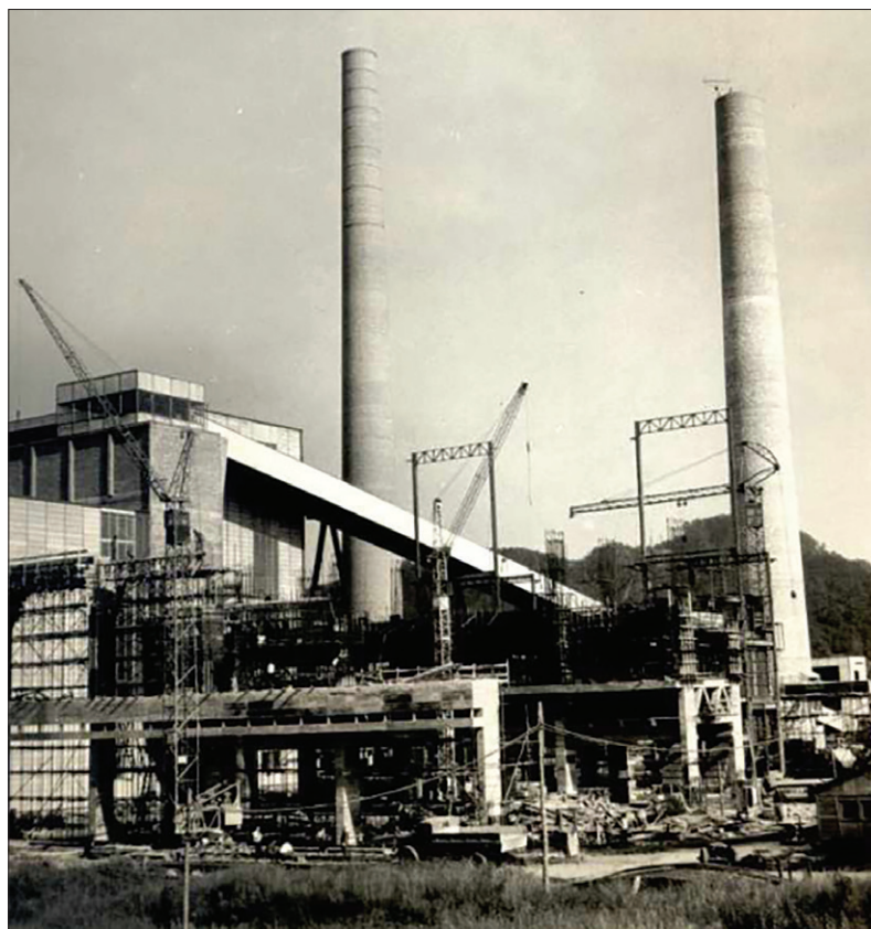
Figure 2.23 TPP Tuzla, Construction of the II stage, 1966
