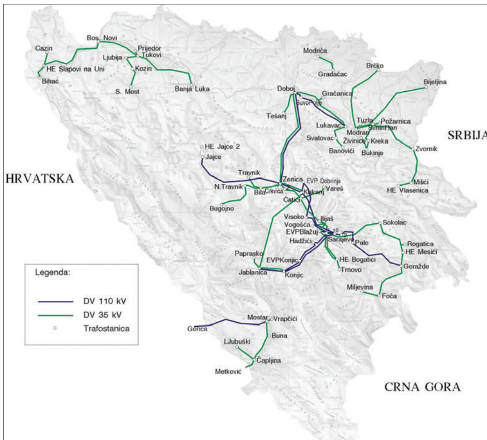
Figure 2.16 110 kV and 35 kV transmission network built by 1954
