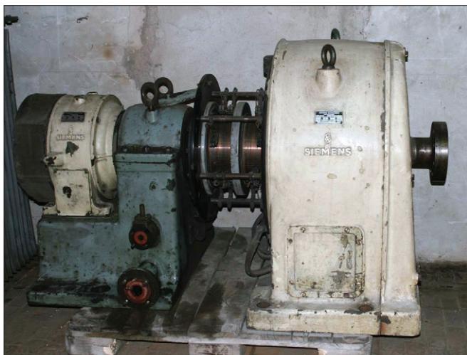
Figure 13.12 Generator exciter 32 MW (production 1956 SIEMENS)
